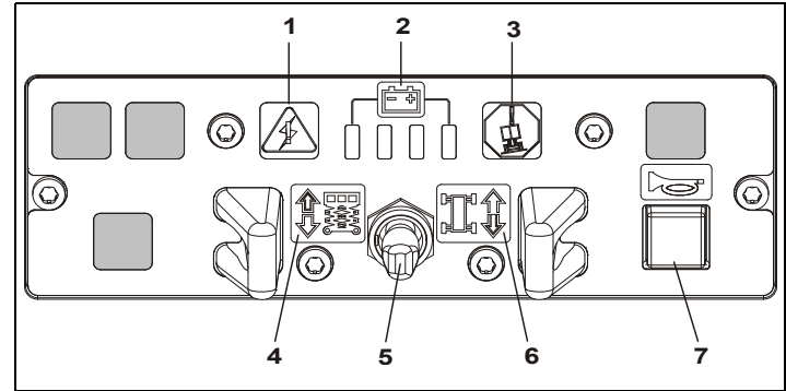
Figur 3-8. Platformens styre-/indikatorpanel
