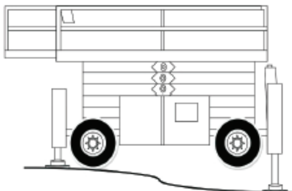
Figur 8.10 - Stabilisatorer
