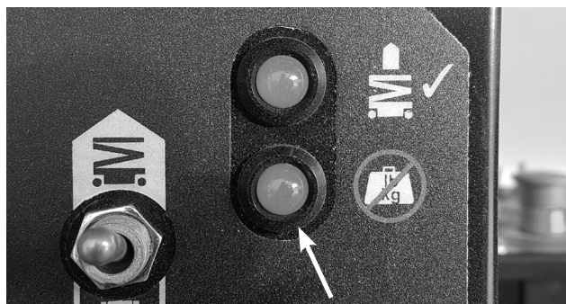
Figur 4.4 - Platform Overbelastningslys
